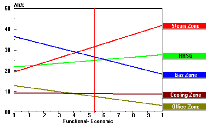
Fig. 7 Gradient Sensitivity
