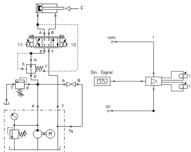
Figure 5. The hydraulic circuit of proportional valve with pressure compensated valve in open loop control actuated by harmonic voltage
