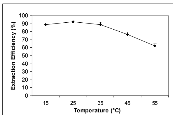
Figure 5. Effects of temperature on the extraction efficiency of PheDH in systems containing PEG-6000 8.5%-(NH 4 ) 2 SO 4 17.5% (pH 8.0).
