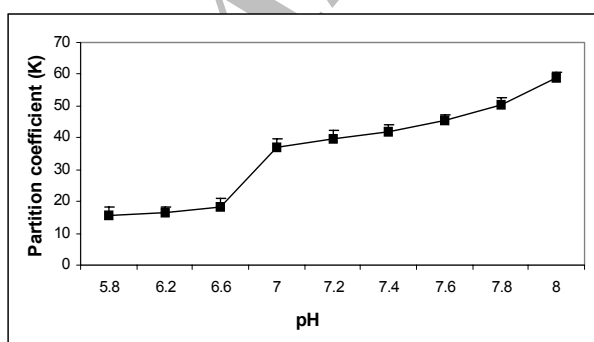
Figure 3. Effects of pH on PheDH partition coefficient ( K ) in PEG-6000 8.5%- (\text{NH}_4)_2\text{SO}_4 17.5% systems.
