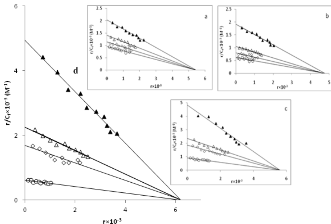
Figure 10. Competition between a-d complexes with ethidium bromide for the binding sites of CT-DNA (Scatchard plot). In curve 1 (▲), Scatchard's plot was obtained with calf thymus DNA alone that its concentration was 60μM. In curves nos. 2(Δ), 3(◇) and 4(○) respectively 50μM, 100μM, 150μM of a, 30μM, 60μM, 90μM of b, 20μM, 40μM, 60μM of c and 10μM, 20μM, 30μM of d complexes at room temperature were added.
