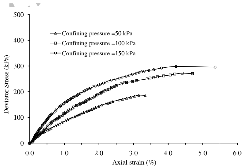
Fig. 8 Stress-strain diagram of layered sample for N=0
