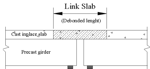
Figure 1. Link slab.
