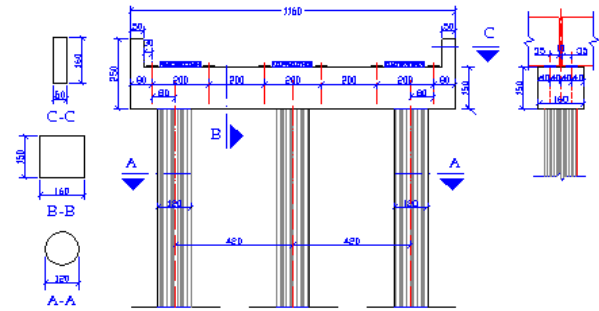
Figure 4. Interior bent.
