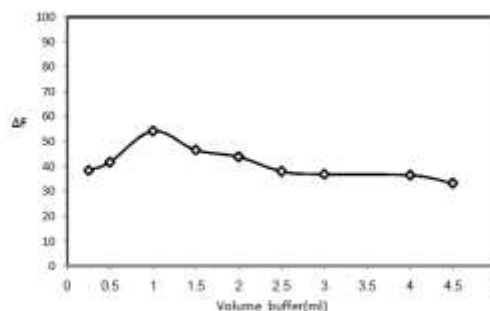
Figure 4. Effect of buffer volume. pH=7.8, [Tb^{3+}] = 5 \times 10^{-4} M, [DFX] = 3 \times 10^{-6} M, [DXR] = 1 \text{ mg L}^{-1} , \lambda_{ex}/\lambda_{em} = 328/545 nm
