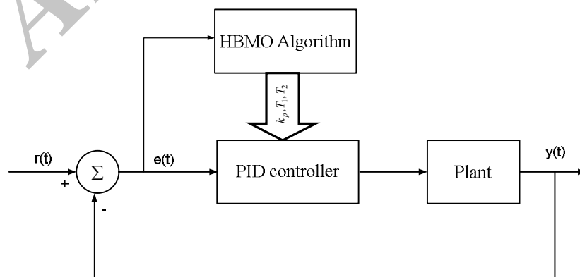
Fig. 3. Schematic of the proposed controller designing
