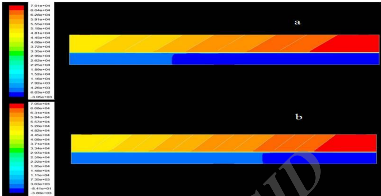
Fig.7. Static pressure contour of baffle-equipped module with 2 cm channel height, 135° baffle angle and 2 mm distance between baffle and membrane surface (a: 8 baffles, b: 12 baffles).
