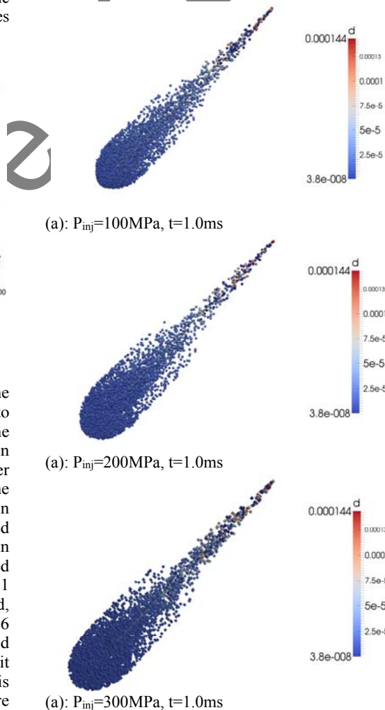
Fig. 17. 3-D plot of spray shapes and droplet sizes.
