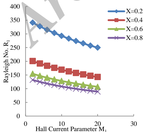
Fig. 5. Variation of Rayleigh number R_1 with Hall current parameter M_1 for G=10, B=10, T_{A_1} = 10, Q_1 = 50, P = 0.1, \epsilon=0.1 for fixed wave numbers x = 0.2, x = 0.4, x=0.6 and x = 0.8 .
