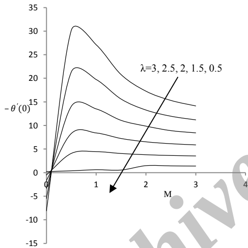
Fig. 8. Nusselt number against magnetic parameter M for various values of \lambda , when Pr=1.0 , \Omega=0.25 , R=0.25 , S=0.4 and \epsilon=0.1 .
