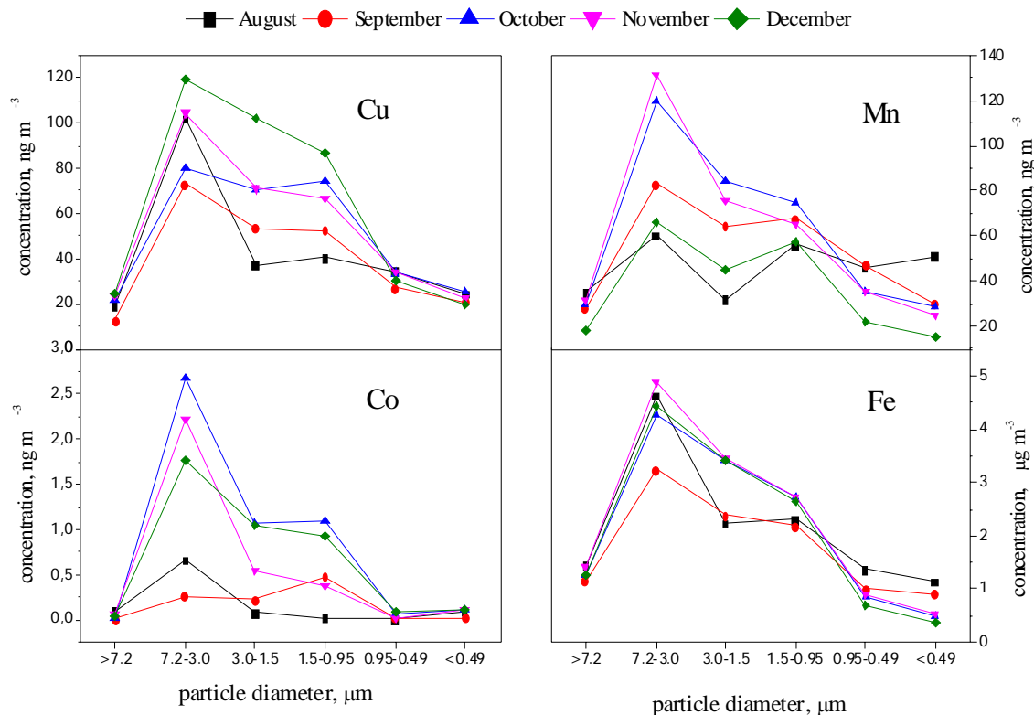
Fig. 1. Mean metal concentration in size fractionated PM for each month
