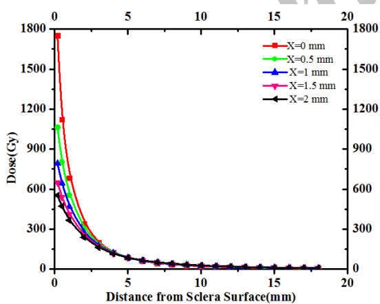
Figure 4 The absorbed dose along the central axis of the plaque.
