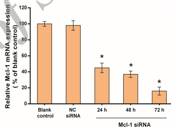
Figure 1. Down-regulation of Mcl-1 mRNA expression by siRNA in HL-60 cells. The cells were transfected with negative control (NC) siRNA or Mcl-1 siRNA for 24, 48 and 72 h. Relative mRNA expression was then measured by qRT-PCR using 2^{-\Delta\Delta Ct} method. The results are expressed as mean \pm SD (n = 3); * P < 0.05 versus blank control and NC siRNA.
