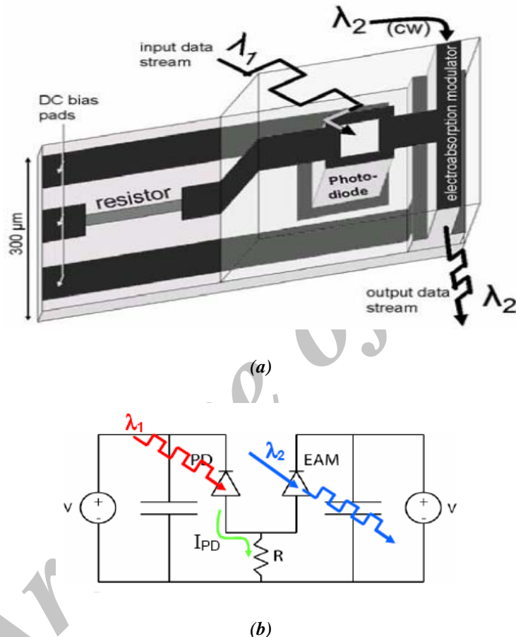
Figure 3. PD/EAM integrated photonic switch: (a) schematic view, (b) a simplified circuit diagram.
