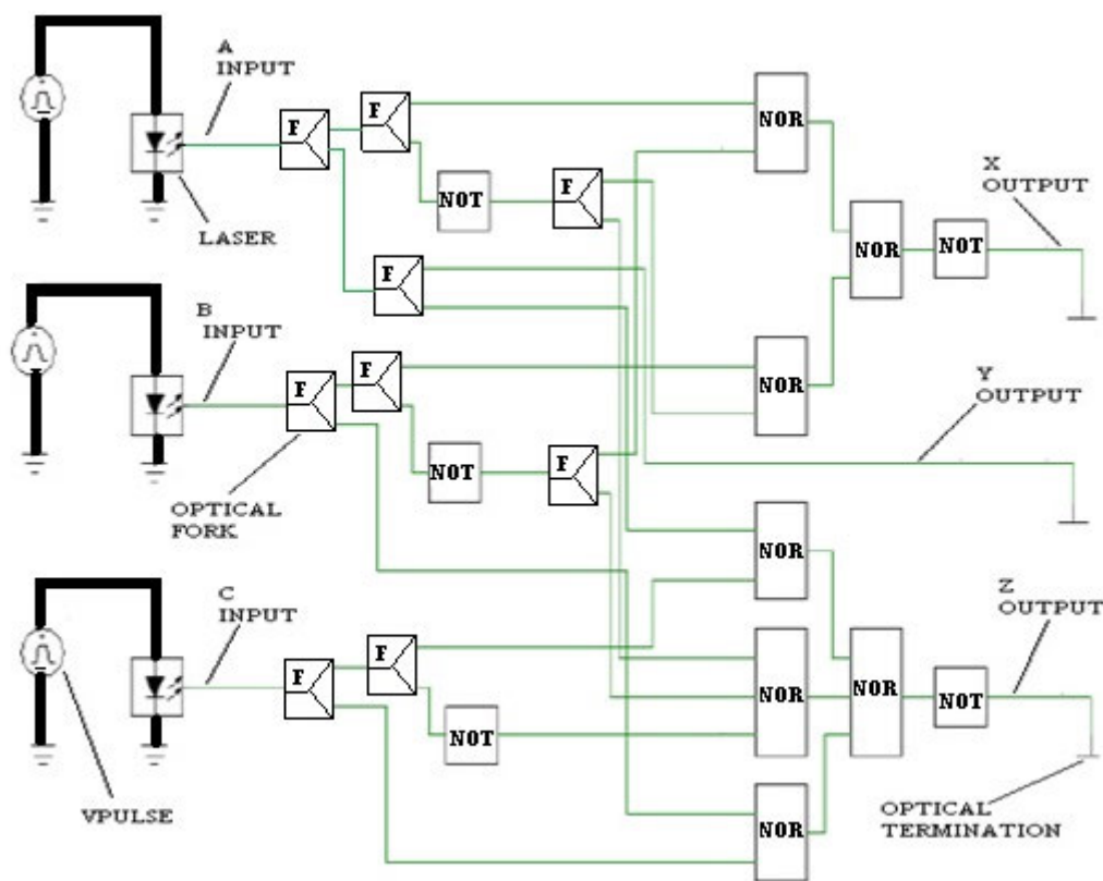
Figure 5. Proposed optical R gate
