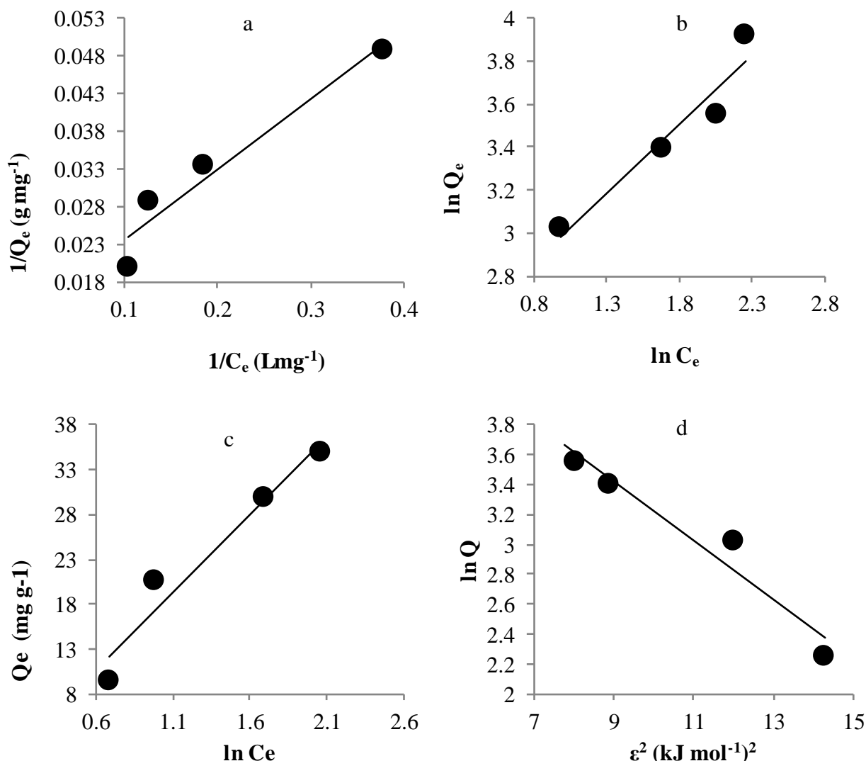
Fig. 7. Isothermal fits for electrocoagulation removal of Bromophenol Blue: (a) Langmuir (b) Freundlich (c) Temkin, (d) Dubinin – Radushkevich.
