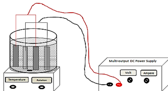
Fig. 2. Laboratory Scale Electrocoagulation Cell.
