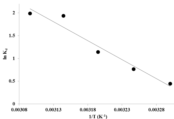
Fig. 11. van't Hoff linear plots of \ln K_d versus 1/T for the electrocoagulation removal of Bromophenol blue dye from aqueous solution.
