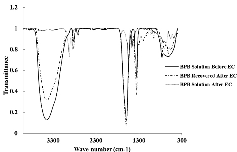
Fig.12. FTIR of the solution of BPB dye solution before and after removal.
