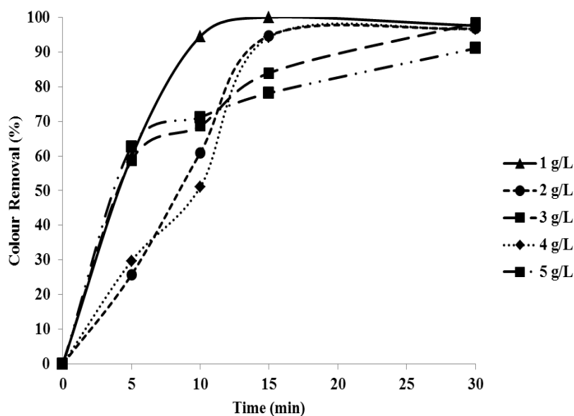
Fig. 5. Effect of electrolyte concentration on % Colour Removal. Dye concentration 50 \text{ mgL}^{-1} , at 30^\circ\text{C} , Current Density: 0.59 \text{ Am}^{-2} and pH 7.
