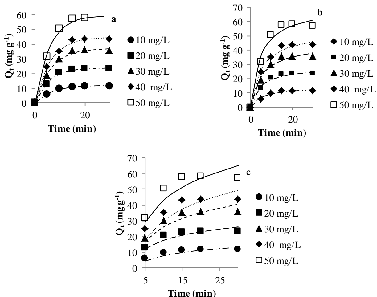
Fig. 8. Kinetic of electrocoagulation removal of Bromophenol Blue (a) Pseudo first-order kinetic (b) Pseudo second-order kinetic and (c) Elovich kinetic model fit. Temp 30 °C, Current Density: 0.59 Am -2 and pH 7.
