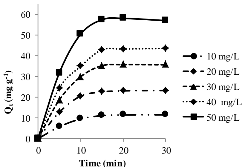
Fig. 6. Effect of initial concentration on the electrocoagulation removal of Bromophenol Blue Dye. Temp 30 °C, Current Density: 0.59 Am -2 and pH 7.
