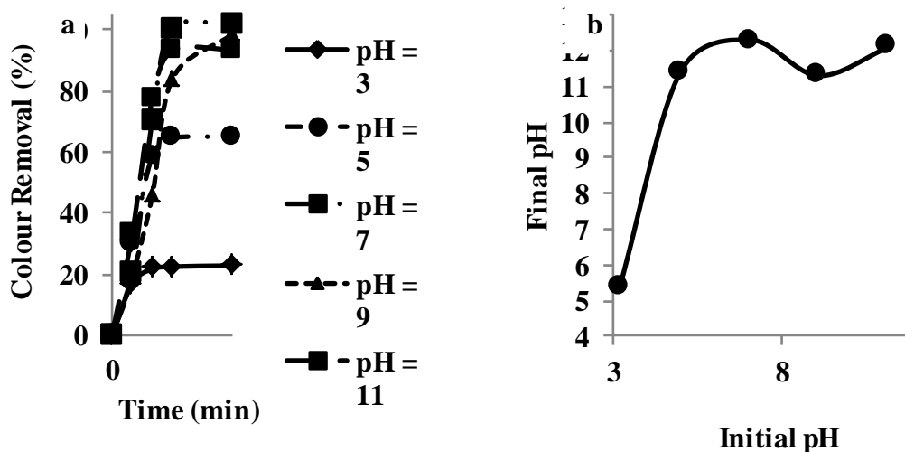
Fig. 4. (a) Effect of initial pH on % Colour Removal (b) Initial and final pH of the dye solution. Dye concentration 50 \text{ mgL}^{-1} , at 30^\circ\text{C} , Current Density: 0.59 \text{ Am}^{-2} and NaCl; 2 \text{ gL}^{-1} .
