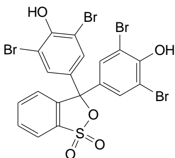
Fig. 1. Structure of Bromophenol Blue
