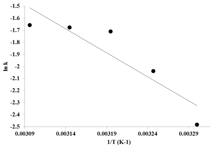
Fig.10. Plot of \ln k vs. 1/T for estimation of Arrhenius parameters for the electrocoagulation removal of Bromophenol blue dye from aqueous solution.
