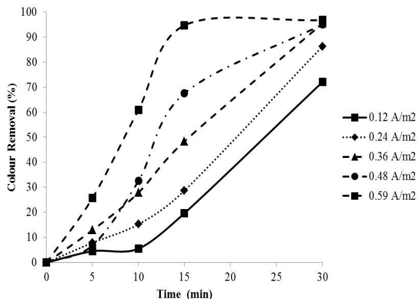
Fig. 3. Effect of current density on % Colour Removal, Dye concentration 50 \text{mg L}^{-1} , at 30 °C, pH 7.0 and NaCl; 2 \text{g L}^{-1} .
