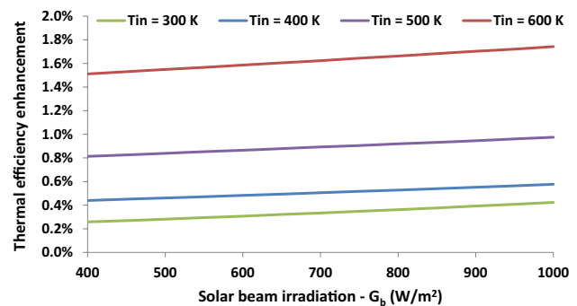
Fig. 15 The impact of the solar beam irradiation on the thermal efficiency enhancement for Nusselt number ratio equal to 2
