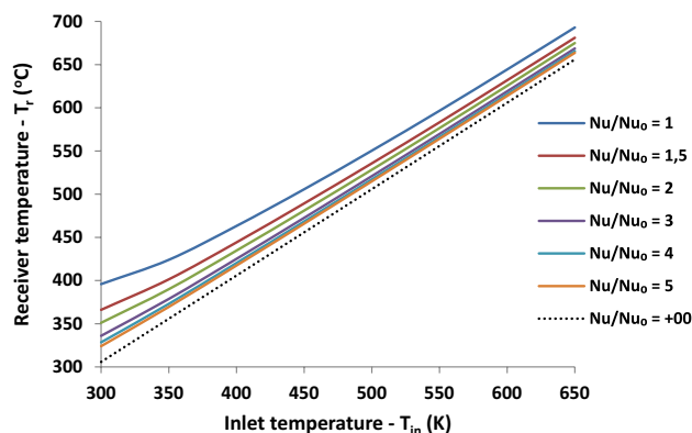
Fig. 5 Receiver temperature for various inlet temperatures and Nusselt number ratios
