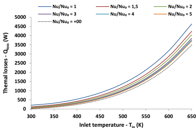
Fig. 4 Thermal losses at various inlet temperatures and Nusselt number ratios
