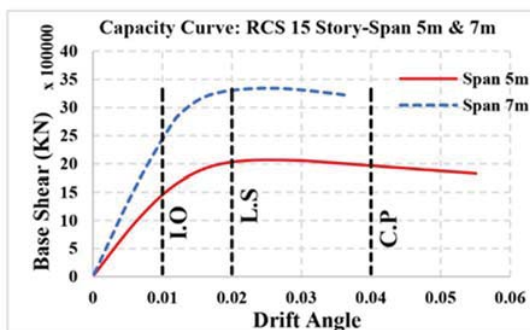
Fig. 3: Capacity curve of RCS 15 story
