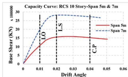
Fig. 4 Capacity curve of RCS 10 story
