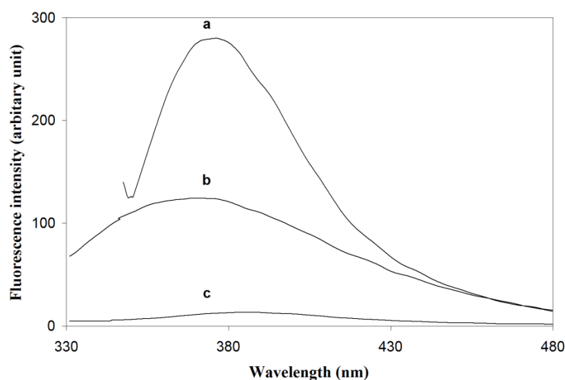
Fig.7. Urine sample spectra with and without DLLME-AgNPs procedure; \lambda_{\text{ex}} 330 nm, slit width 15 nm; \lambda_{\text{em}} 376 nm, slit width 15 nm. (a) Spectrum of THD ( 20 \text{ ng mL}^{-1} ) in urine treated by DLLME-AgNPs; (b) spectrum of urine alone; (c) Spectrum of urine alone treated by DLLME-AgNPs.
