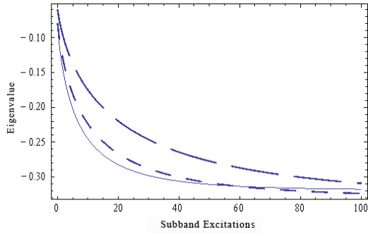
Fig. 2. Eigenvalue versus subband excitations at \tau=2 for different Rashba parameters: \alpha=1.6\times 10^{-11} eVm ( long-dashed line), \alpha=2.4\times 10^{-11} eVm (short-dashed line) and \alpha=3.2\times 10^{-11} eVm (solid line)
