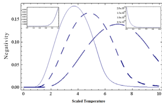
Fig. 6. Graphs of negativity versus the scaled temprature, \tau , for a magnetic field of 5.69 Tesla and different Rashba parameters. Left (right) inset depicts the negativity for small (large) \tau 's
