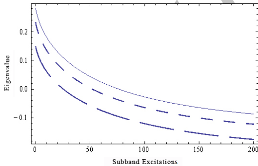
Fig. 4. Eigenvalue versus subband excitations at \tau=10 , for different Rashba parameters: \alpha=1.6\times 10^{-11} eVm ( long-dashed line), \alpha=2.4\times 10^{-11} eVm (short-dashed line) and \alpha=3.2\times 10^{-11} eVm (solid line)
