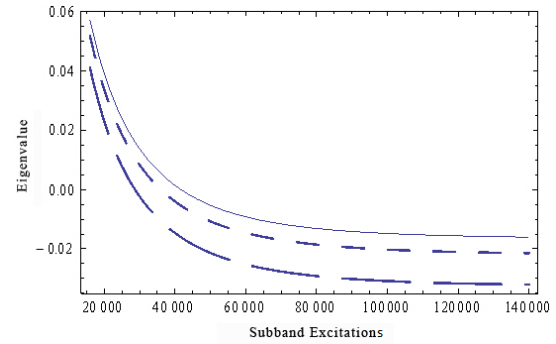
Fig. 5. Eigenvalue versus subband excitations at \tau=100 , for different Rashba parameters: \alpha=1.6\times 10^{-11} eVm ( long-dashed line), \alpha=2.4\times 10^{-11} eVm (short-dashed line) and \alpha=3.2\times 10^{-11} eVm (solid line)
