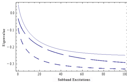
Fig. 3. Eigenvalue versus subband excitations at \tau=4 , for different Rashba parameters: \alpha=1.6\times 10^{-11} eVm ( long-dashed line), \alpha=2.4\times 10^{-11} eVm (short-dashed line) and \alpha=3.2\times 10^{-11} eVm (solid line)
