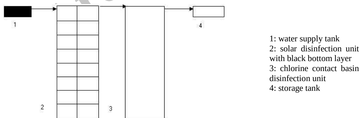
Figure 2: schematic flow diagram for combined solar – chlorine disinfection process
