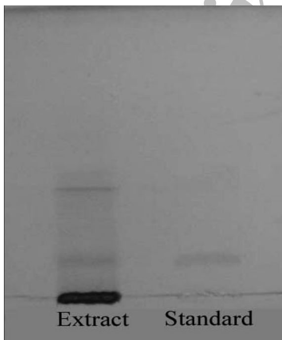
Figure 1. The TLC chromatogram of the licorice extract and 18 \beta -glycyrrhetic acid standard
