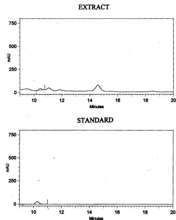
Figure 3. Stacked plots of HPLC chromatograms of the 18 \beta -glycyrrhetic acid in standard and extract samples
