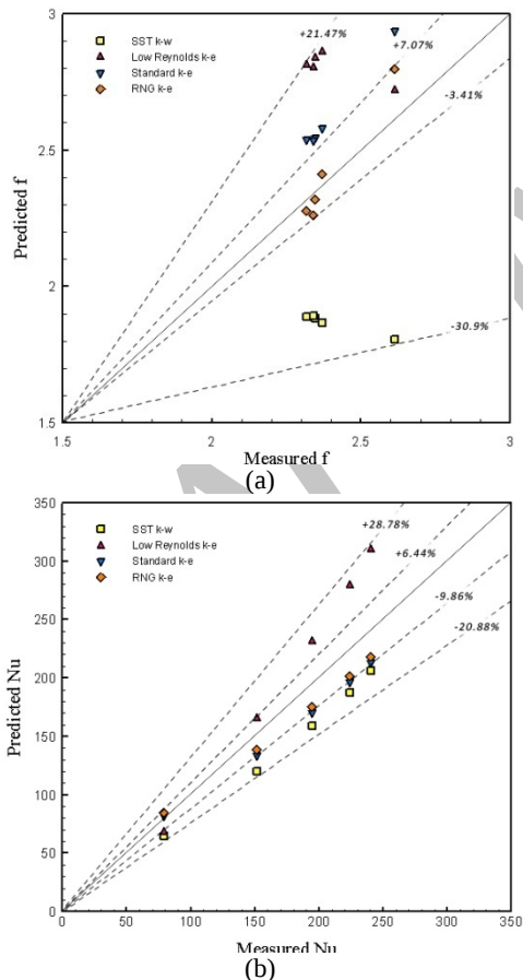
Figure 6. Experimental measured f_c versus numerical predicted f_c (a) and measured \overline{Nu}_c versus numerical predicted \overline{Nu}_c (b).
