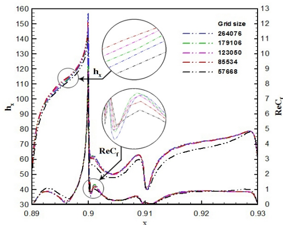
Figure 2. The effect of grid densities on local convective heat transfer coefficient and skin-friction coefficient for eighth rib at Re = 23000 .
