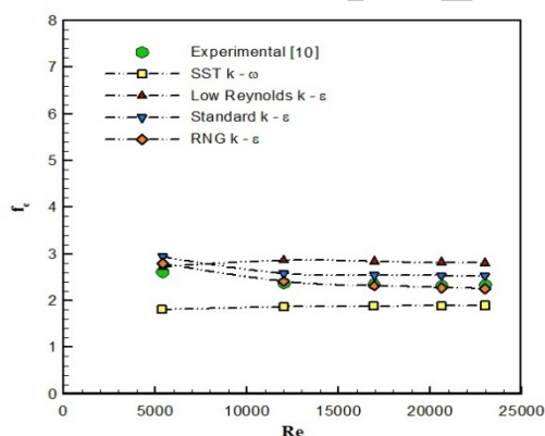
Figure 4. The comparison between friction factors for different turbulent models.
