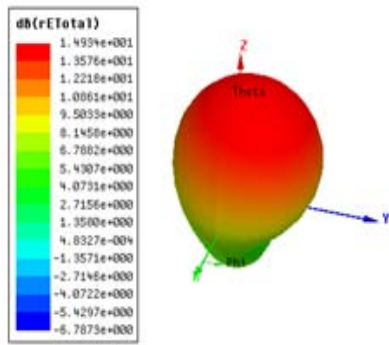
Figure 4. The illustration of the polar plot of Zero Order Fractal
