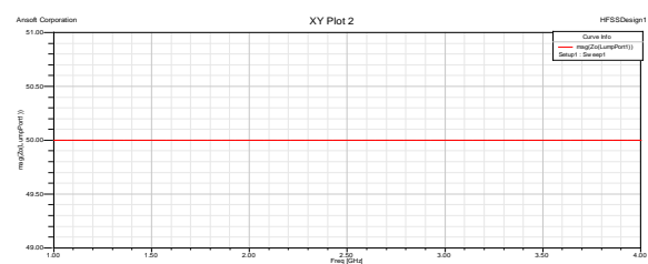
Figure 13. Port Impedance for the designed antenna
