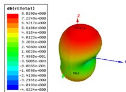
Figure 12. The illustration of the polar plot of Second Order Fractal
