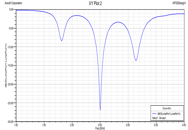
Figure 2. The return loss ( S_{11} , dB) versus frequency (GHz) plot for initiator
