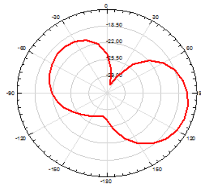
Figure 11. Radiation Pattern for Second Order Fractal
