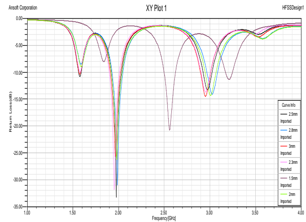
Figure 17. Effect of Feed Width
