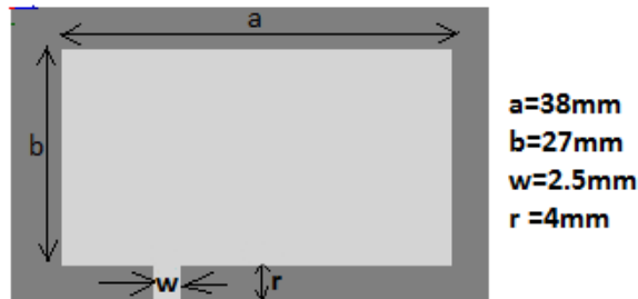
Figure 1. The Microstrip patch antenna (Initiator)
