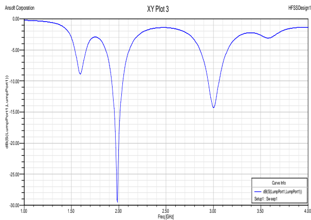
Figure 6. The return loss ( S_{11} , dB) versus frequency (GHz) plot for First Order Fractal
