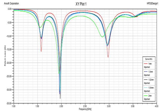
Figure 16. Effect of Substrate Height
