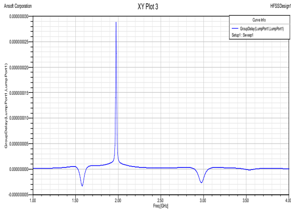
Figure 14. Group Delay for the final antenna design
