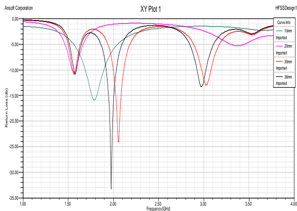
Figure 18. Effect of Ground Length
