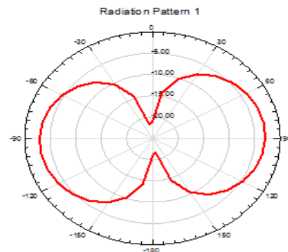
For E plane theta=0degree
