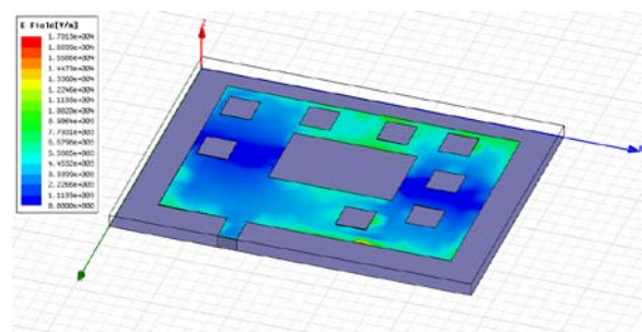
Figure 12. Current Distribution for Second Order Fractal
