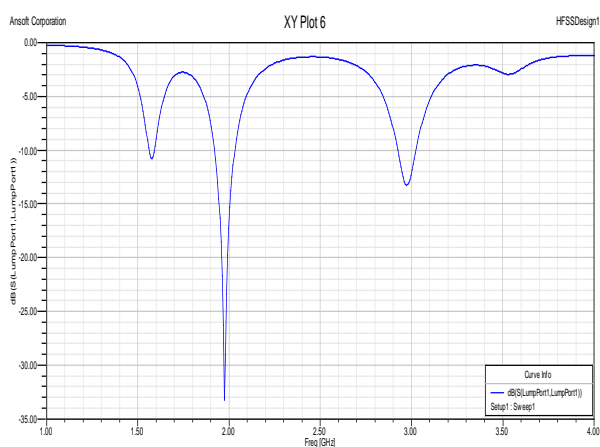
Figure 10. The return loss ( S_{11} , dB) versus frequency (GHz) plot for Second Order Fractal
