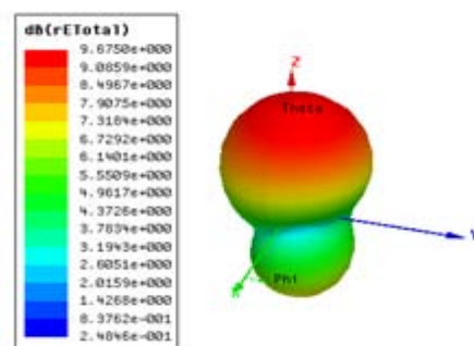
Figure 8. The illustration of the polar plot of First Order Fractal
