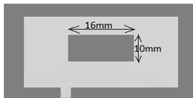
Figure 5. The First Order Fractal Microstrip antenna
