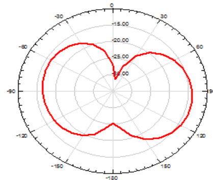
Figure 7. Radiation Pattern for First Order Fractal
