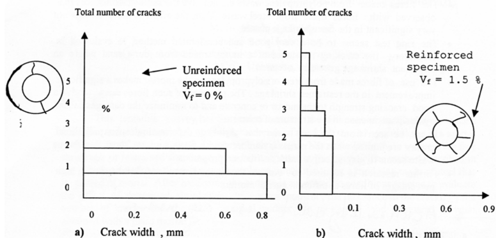
Figure 5 Typical example from the tests showing the number of cracks, crack widths of unreinforced (a) and reinforced mortar with fibrous waste of polypropylene (b)
